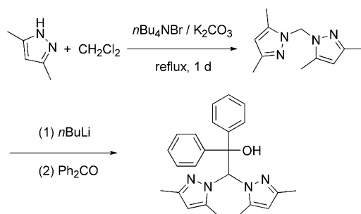
Scheme 1. Synthesis of heteroscorpionate ligand precursor.
