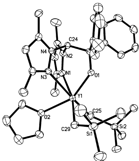
Figure 3. ORTEP drawing of complex 2 with thermal ellipsoids at 35% probability levels. The hydrogen atoms and the free THF molecule are omitted for clarity.
