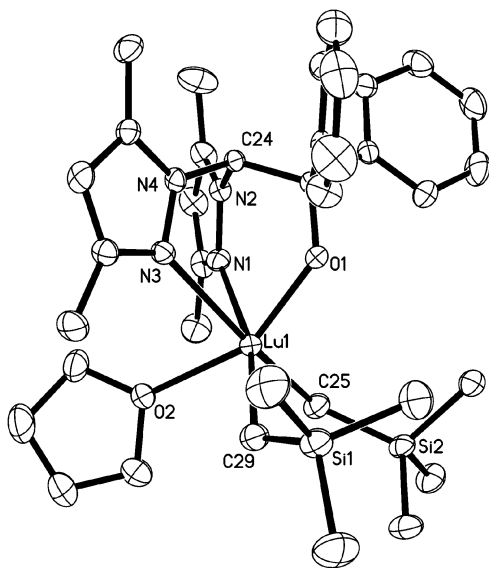
Figure 4. ORTEP drawing of complex 3 with thermal ellipsoids at 35% probability levels. The hydrogen atoms and the free THF molecule are omitted for clarity.
