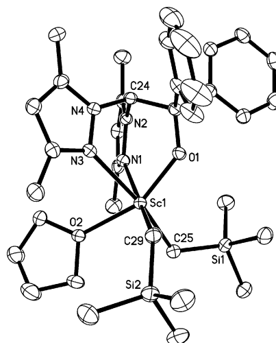
Figure 2. ORTEP drawing of complex 1 with thermal ellipsoids at 35% probability levels. The hydrogen atoms and the free THF molecule are omitted for clarity.
