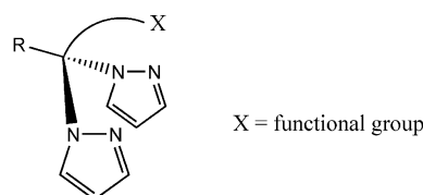
Figure 1. Structure of the heteroscorpionate ligand.
