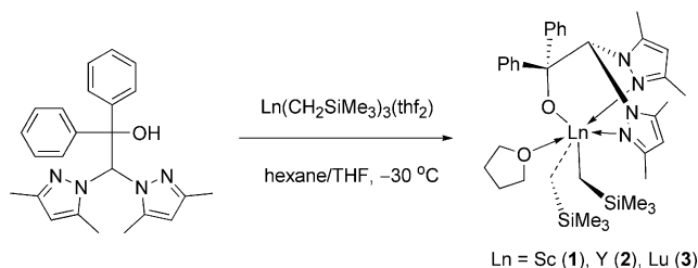
Scheme 2. Preparation of heteroscorpionate rare-earth metal dialkyl complexes 1 , 2 and 3 .
